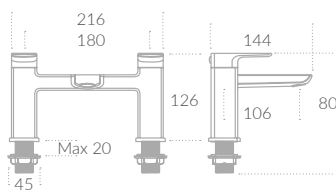
Divine Bath Filler
