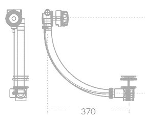
Bath Waste with Overflow Pop Up Waste
