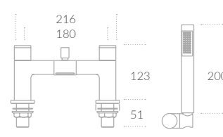
Razo Bath Shower Mixer
